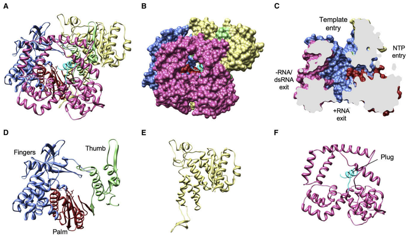
Figure 1. Structure of the VP1 Apoenzyme
