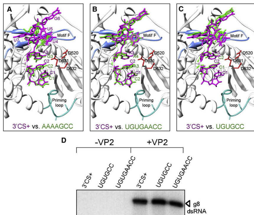
Figure 3. Structure of VP1 in Complex with RNA Oligonucleotides
