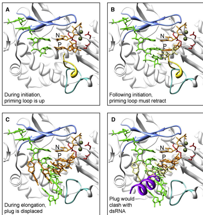
Figure 6. Proposed Model of RNA Synthesis by VP1
