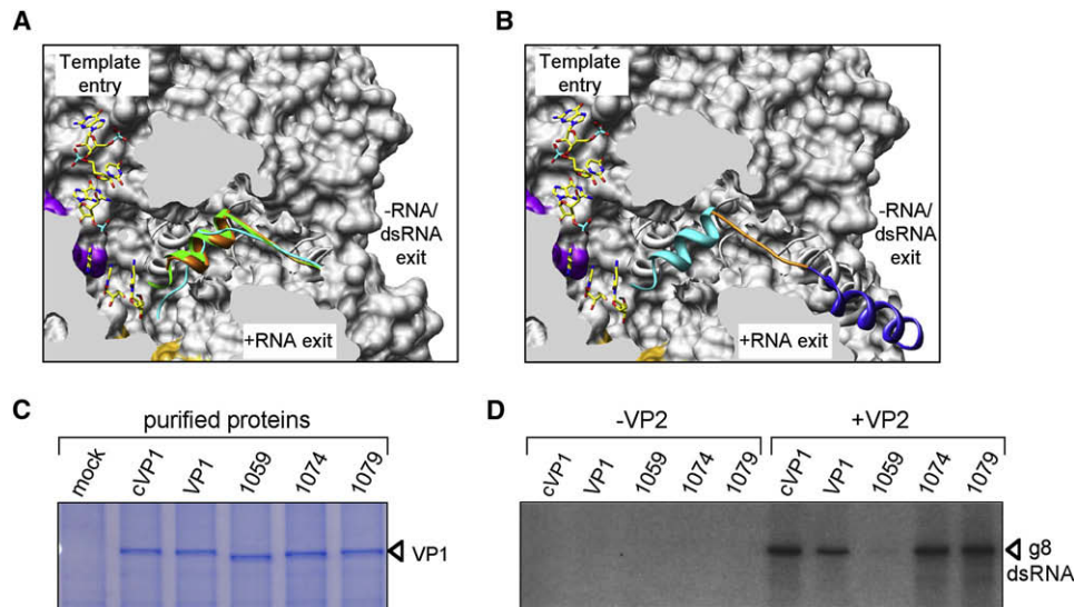
Figure 2. Polymerase Activity of VP1 Plug Mutants
